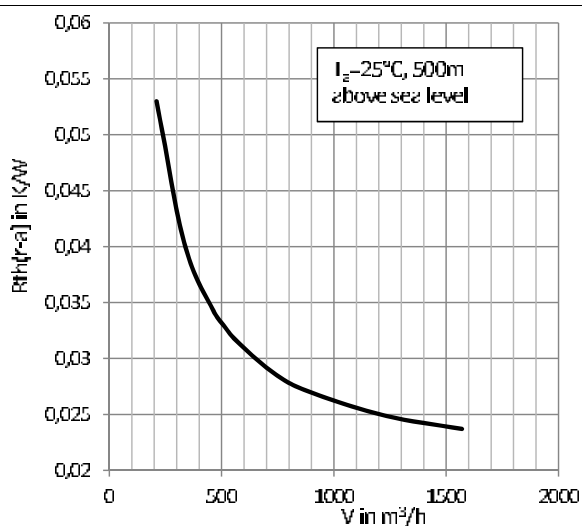
Fig. 9: Thermal resistance R_{th}(r-a) versus flow rate V
